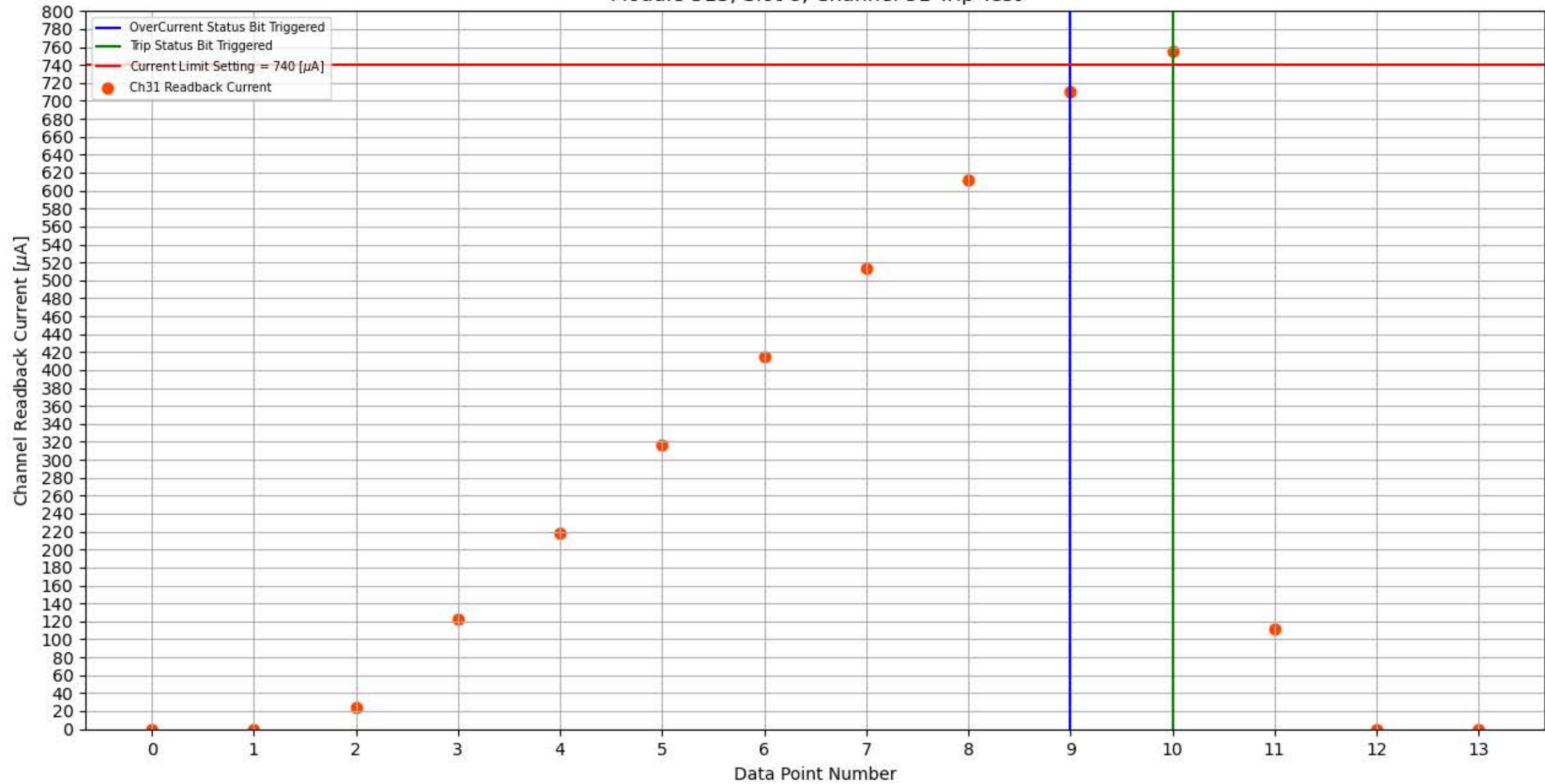
Module 313, Slot 8, Channel 31 Trip Test
