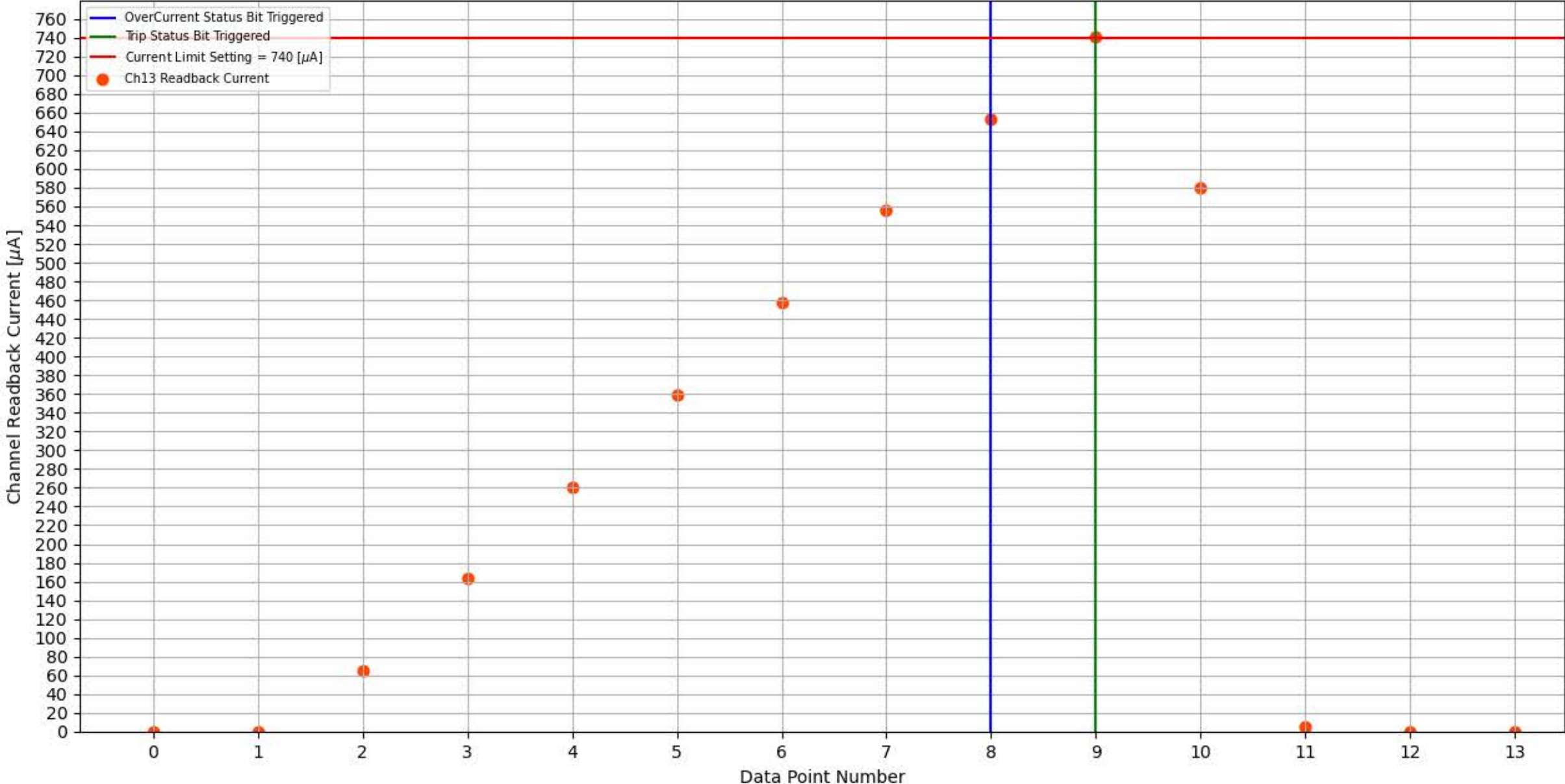
Module 313, Slot 8, Channel 13 Trip Test
