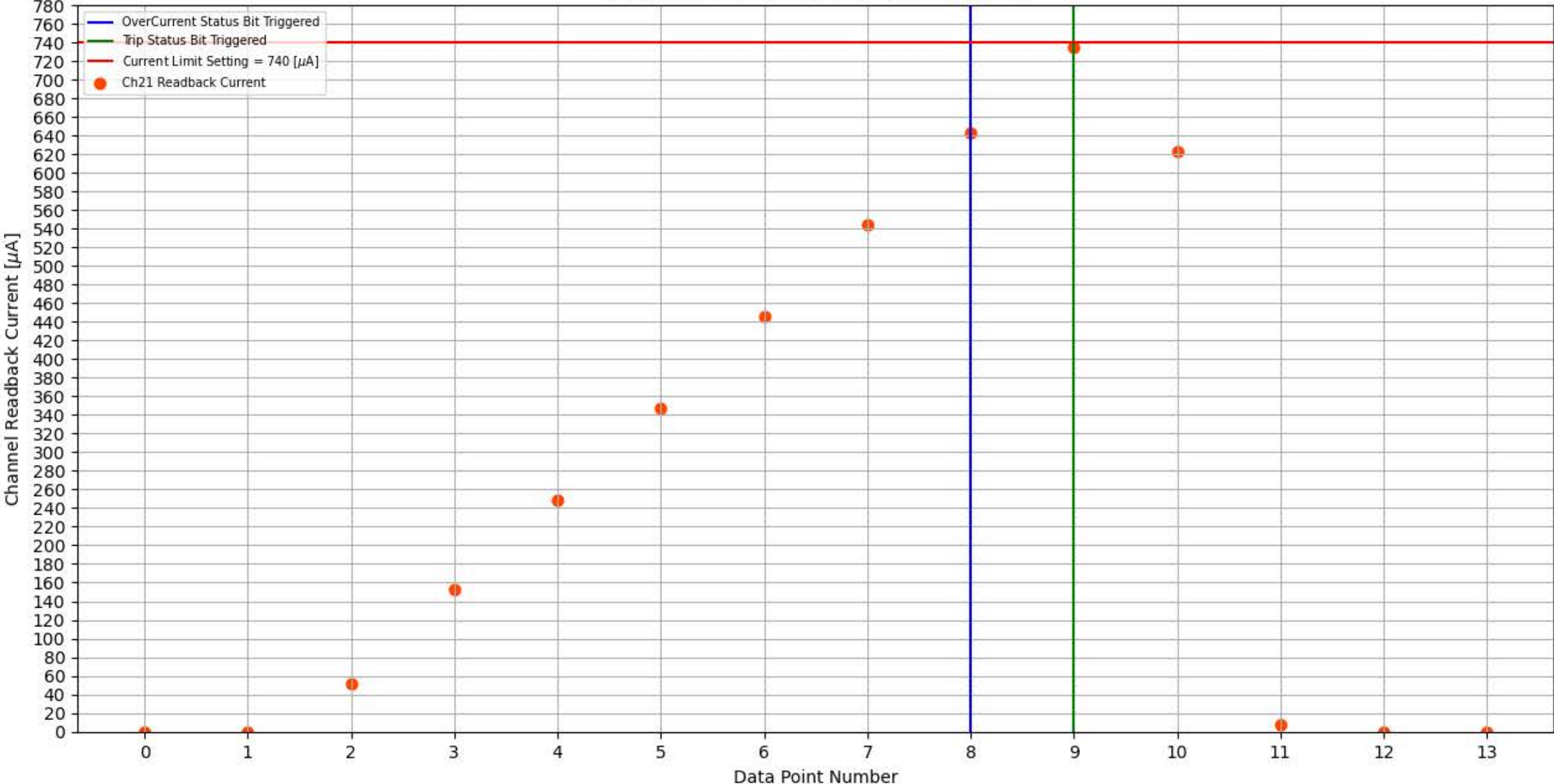
Module 313, Slot 8, Channel 21 Trip Test
