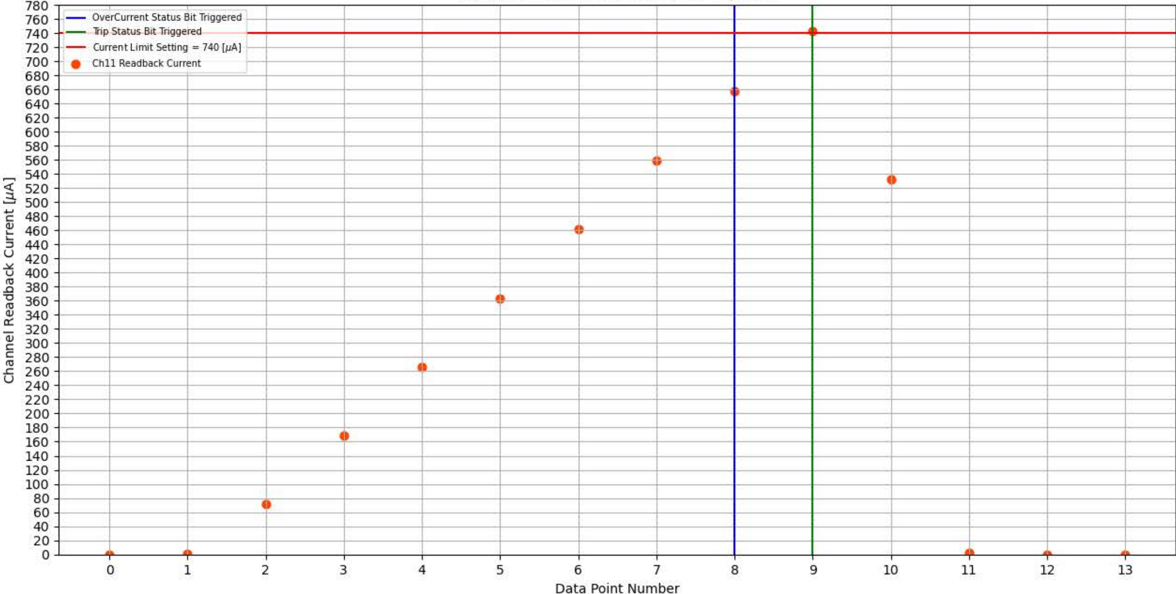
Module 313, Slot 8, Channel 11 Trip Test
