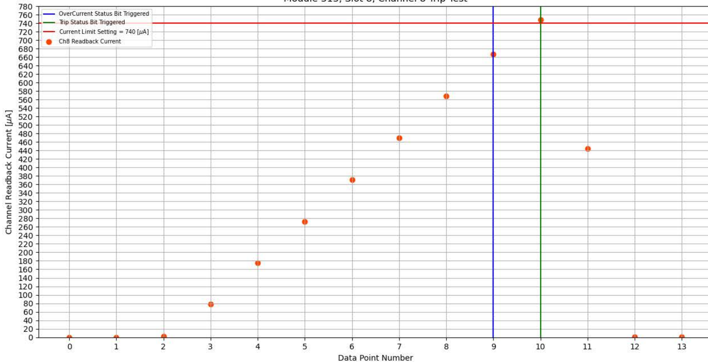
Module 313, Slot 8, Channel 8 Trip Test
