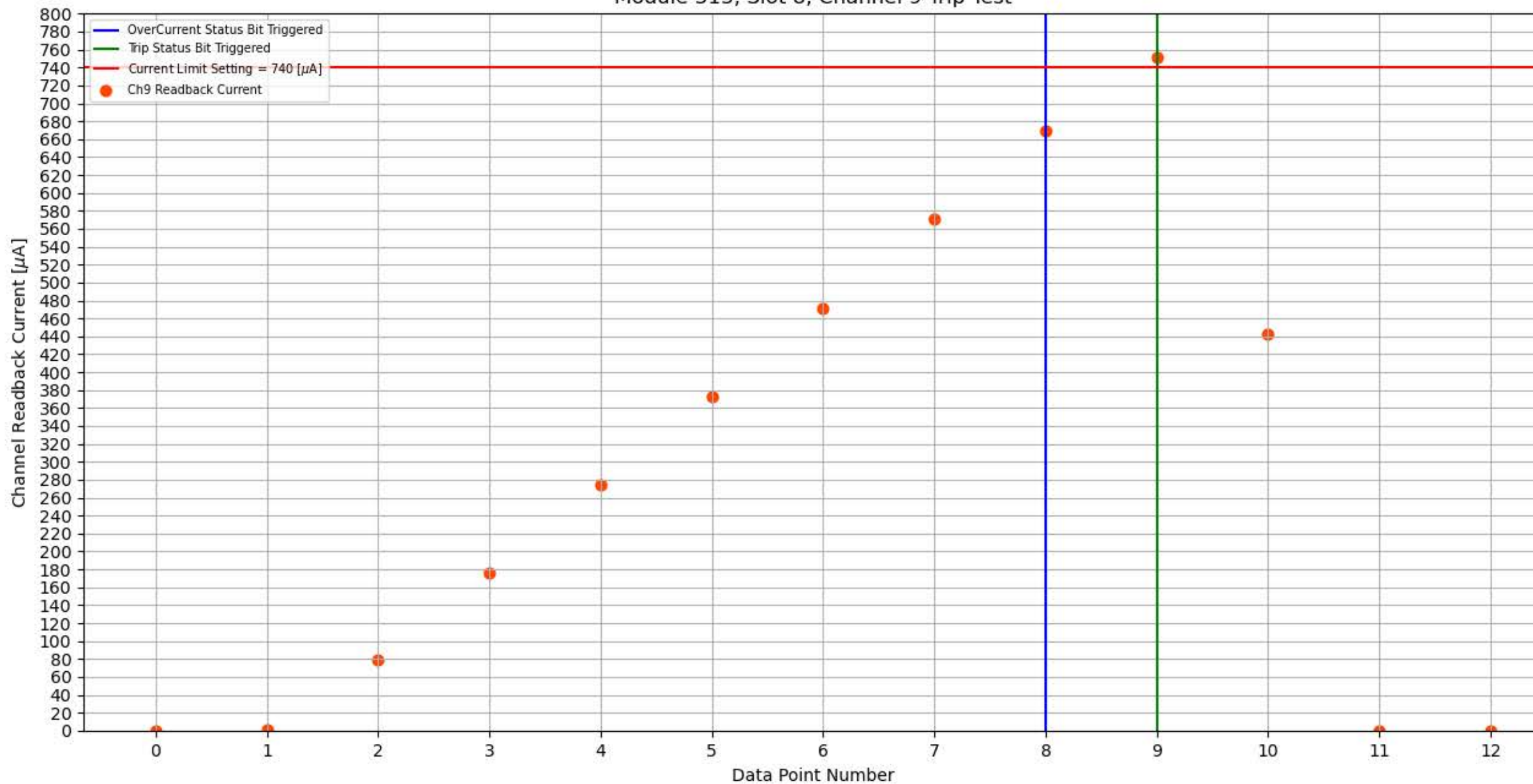
Module 313, Slot 8, Channel 9 Trip Test
