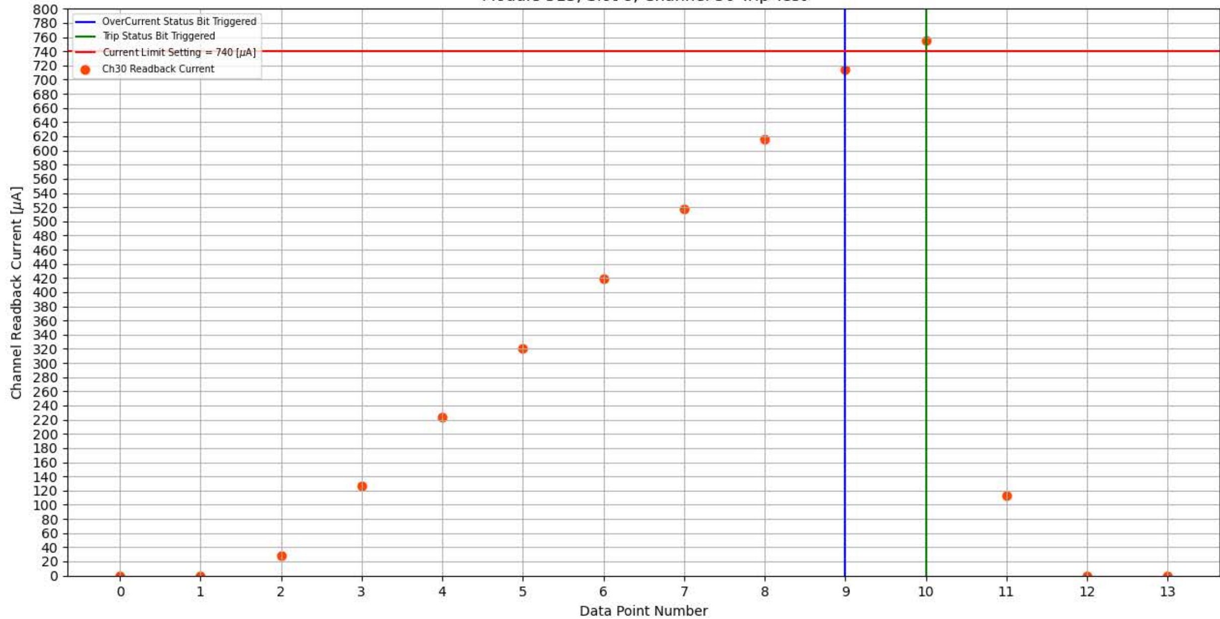
Module 313, Slot 8, Channel 30 Trip Test
