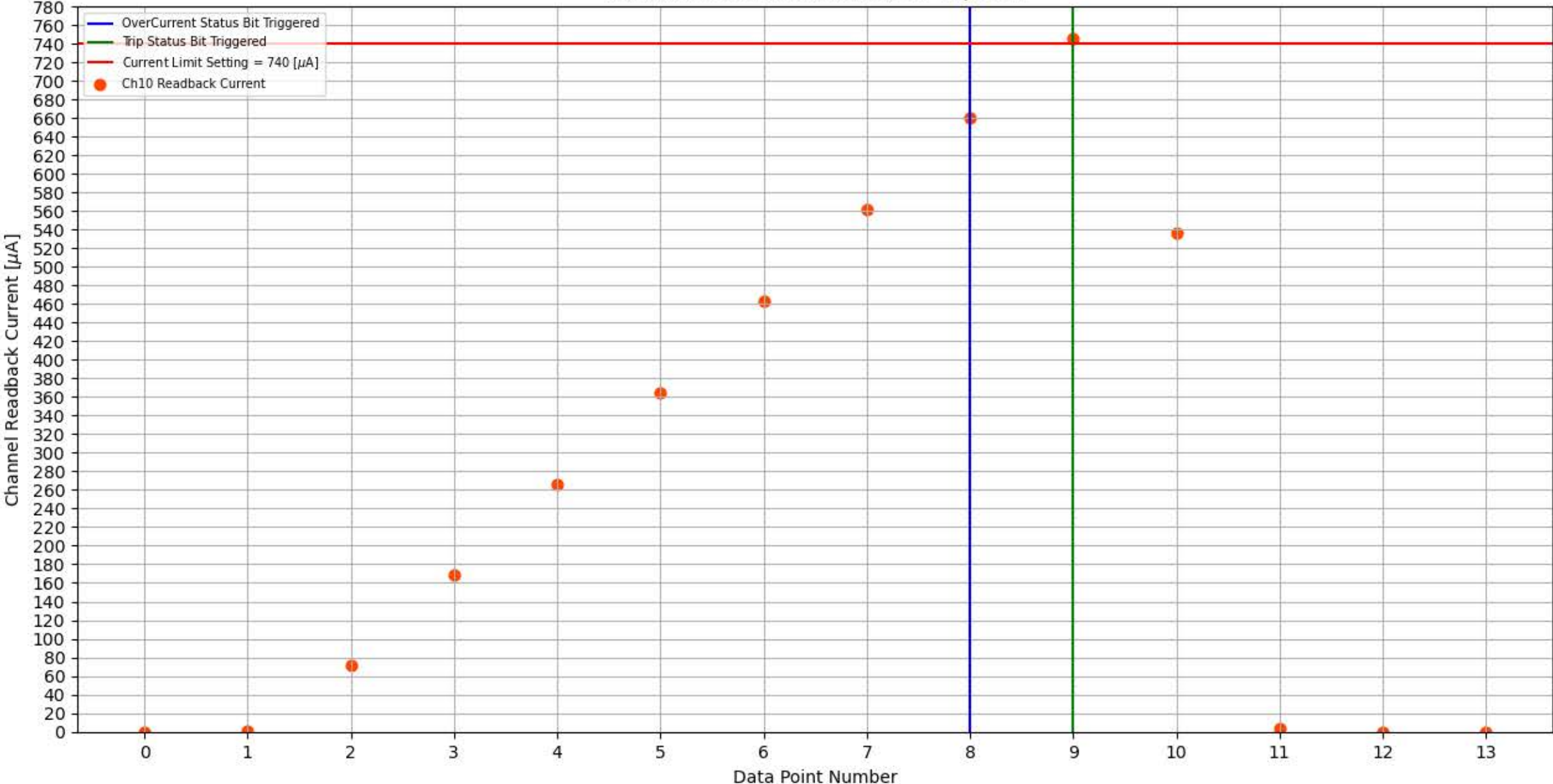
Module 313, Slot 8, Channel 10 Trip Test
