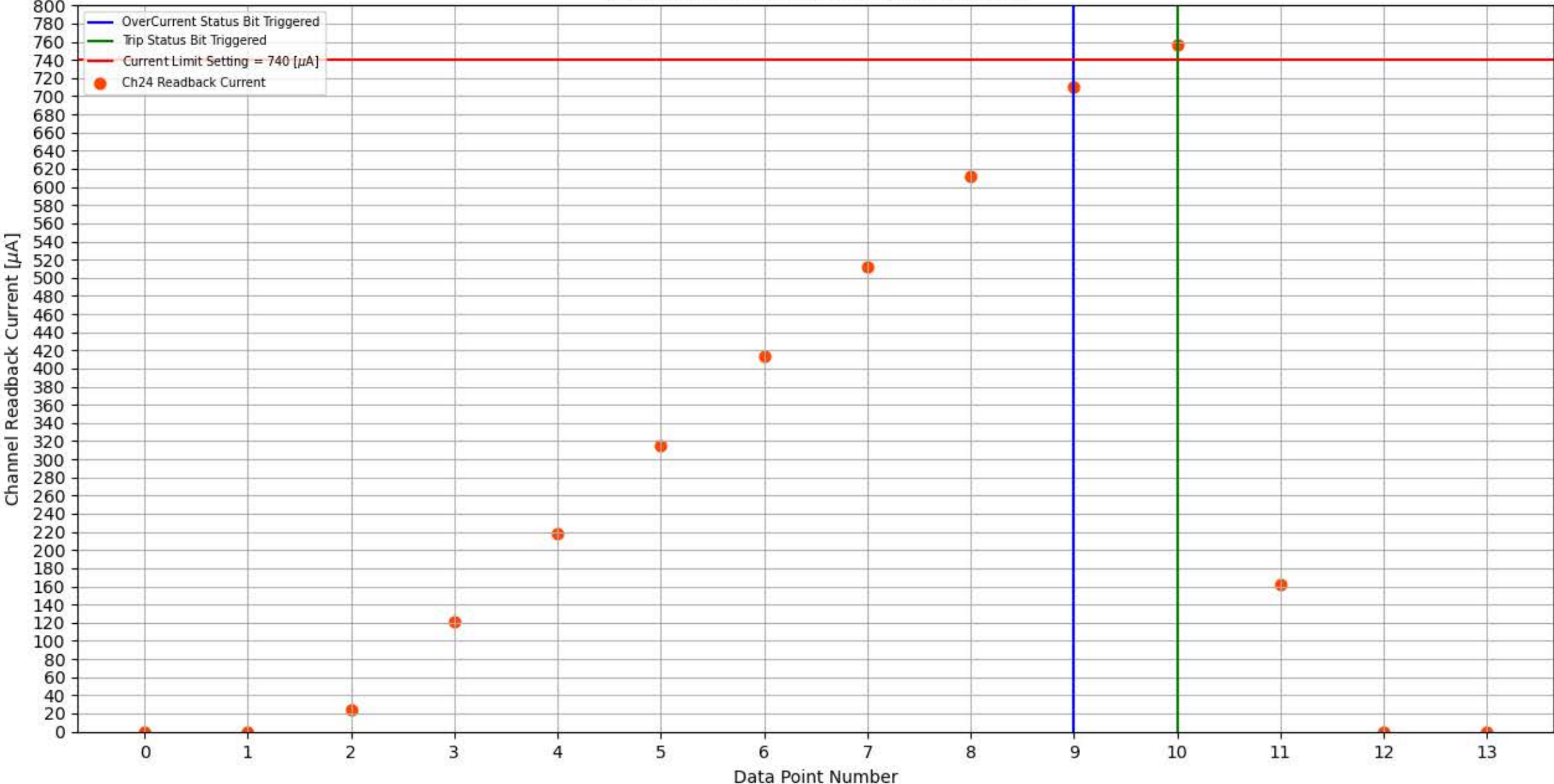
Module 313, Slot 8, Channel 24 Trip Test
