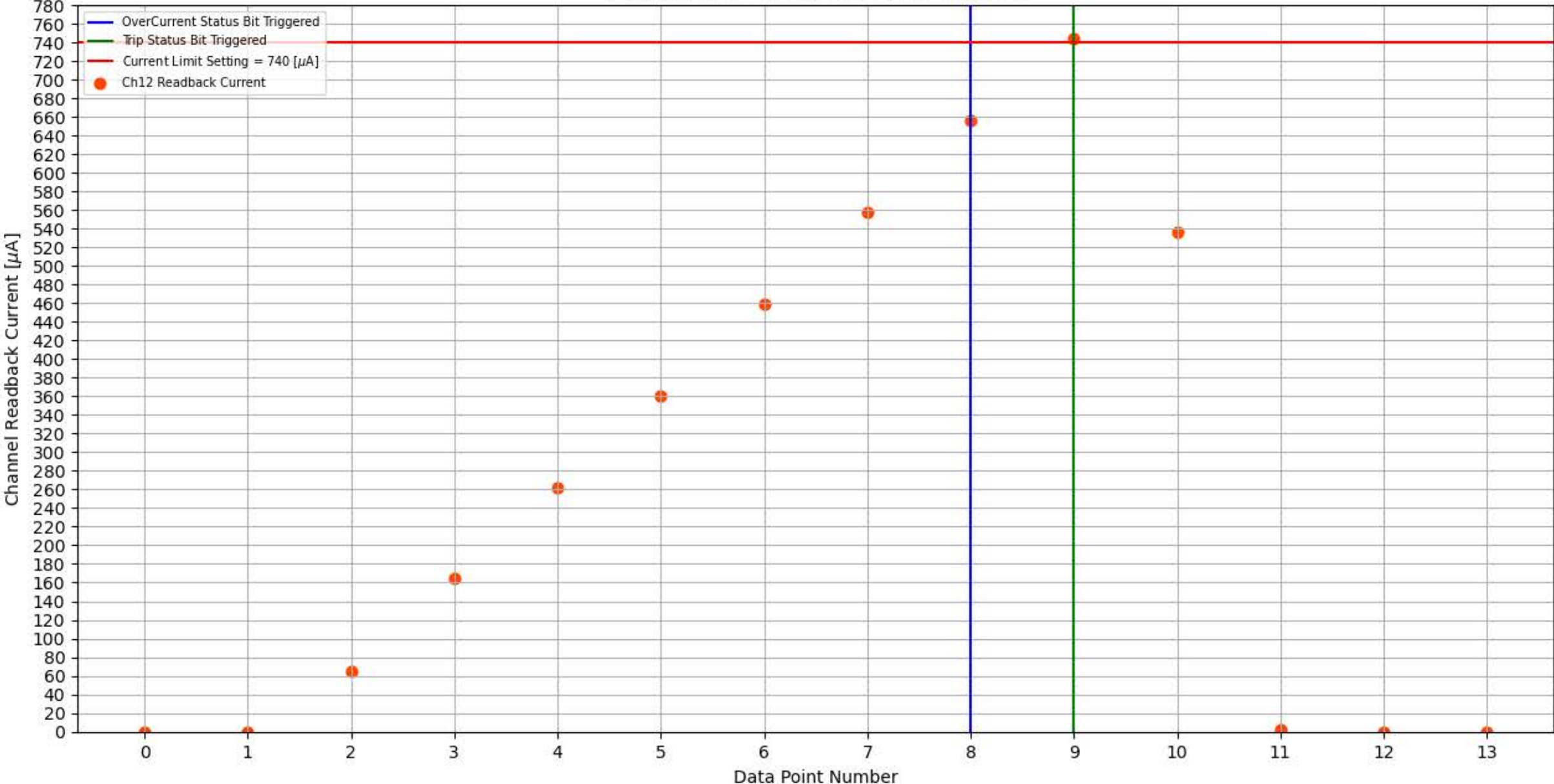
Module 313, Slot 8, Channel 12 Trip Test
