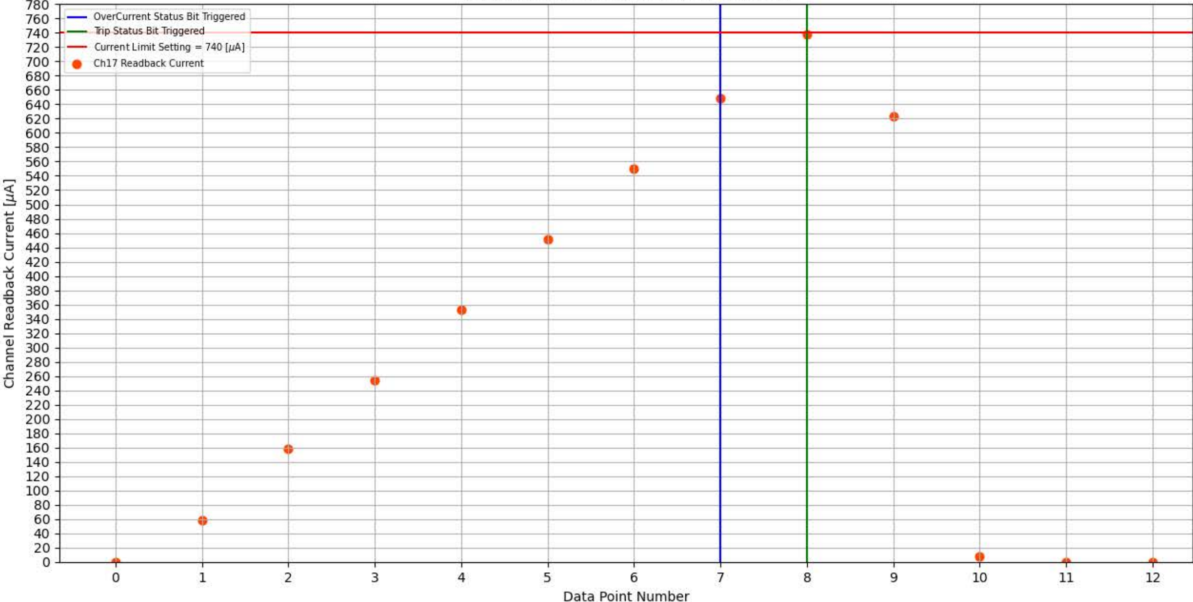
Module 313, Slot 8, Channel 17 Trip Test
