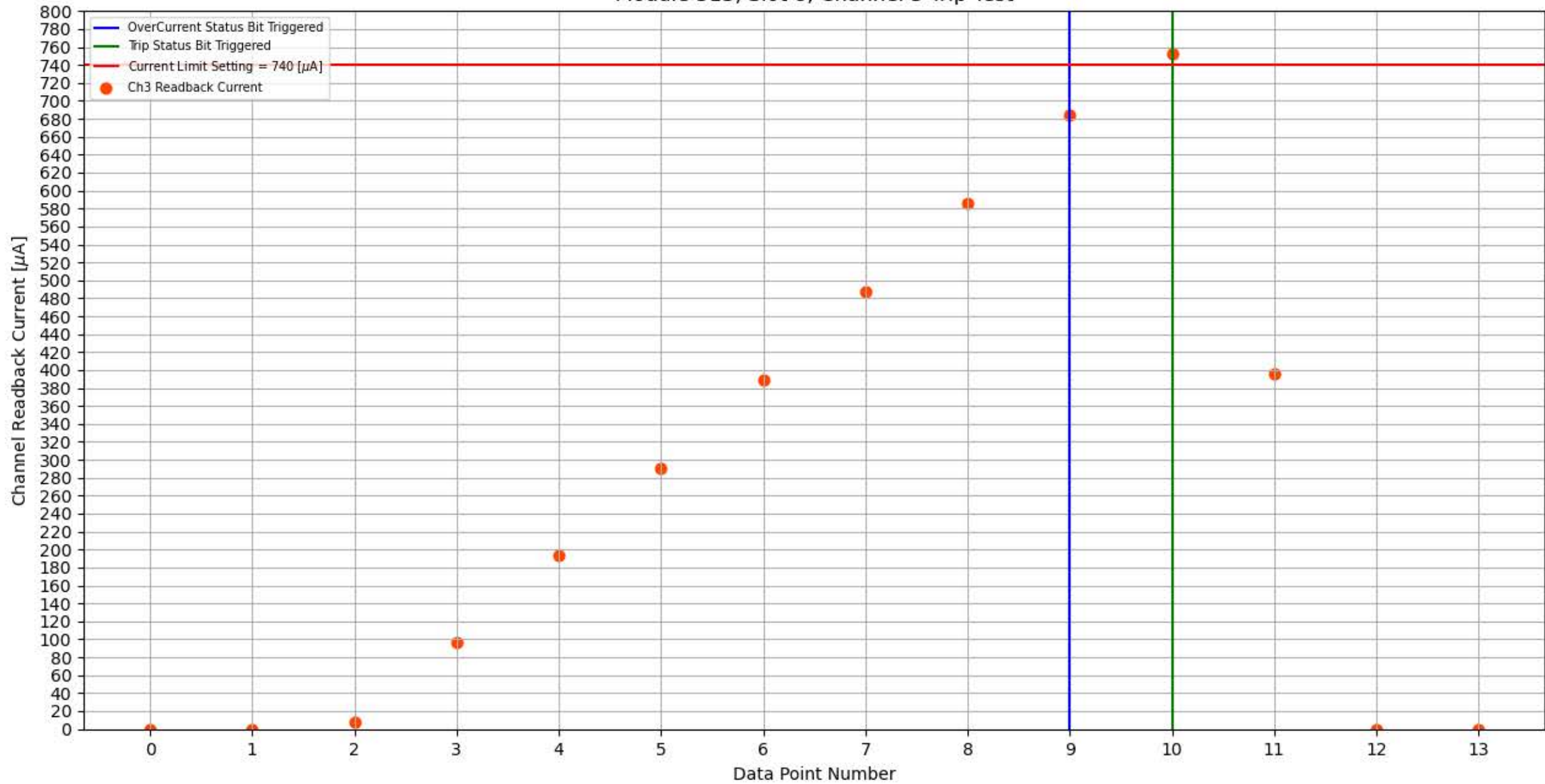
Module 313, Slot 8, Channel 3 Trip Test
