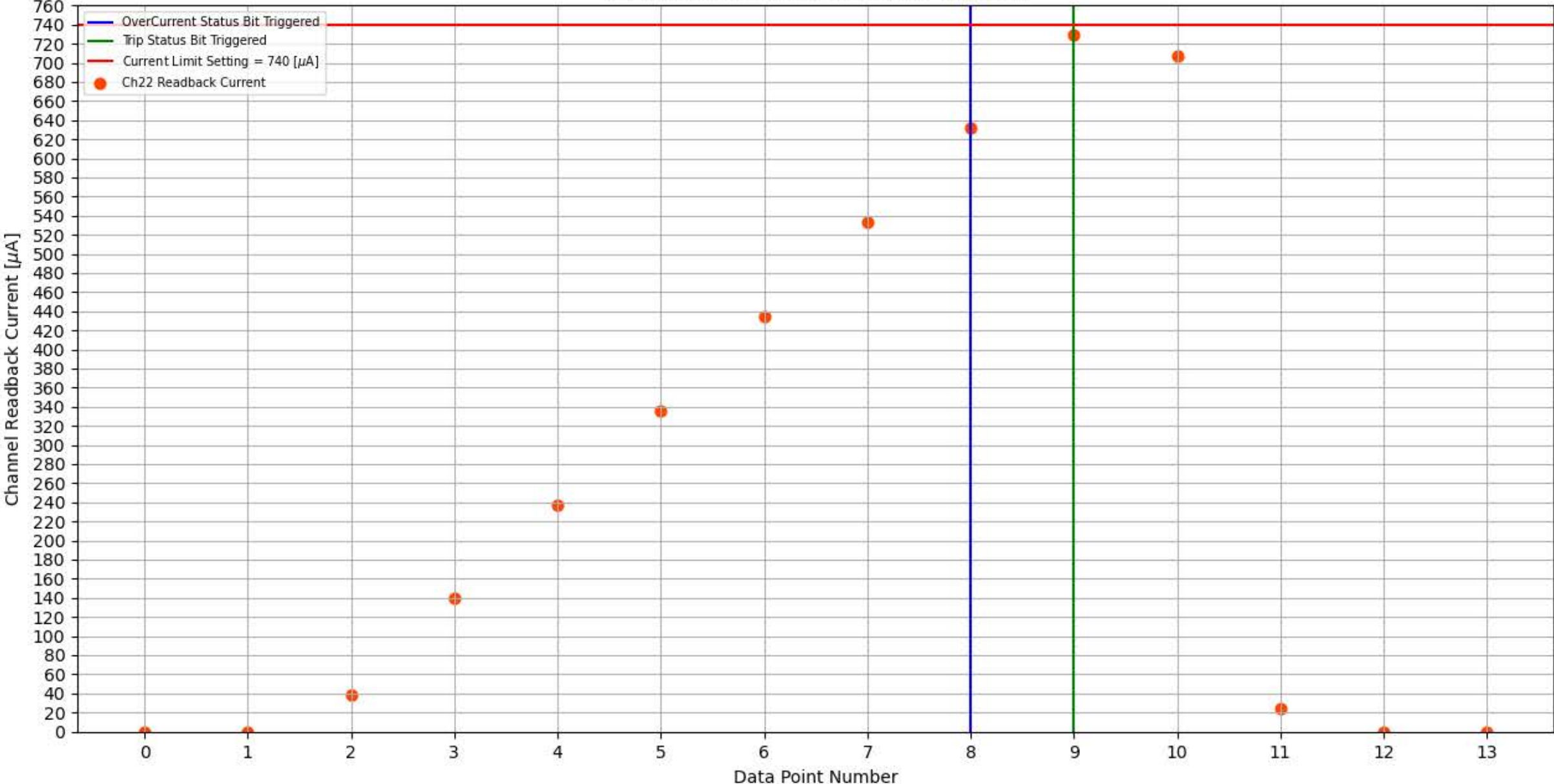
Module 313, Slot 8, Channel 22 Trip Test
