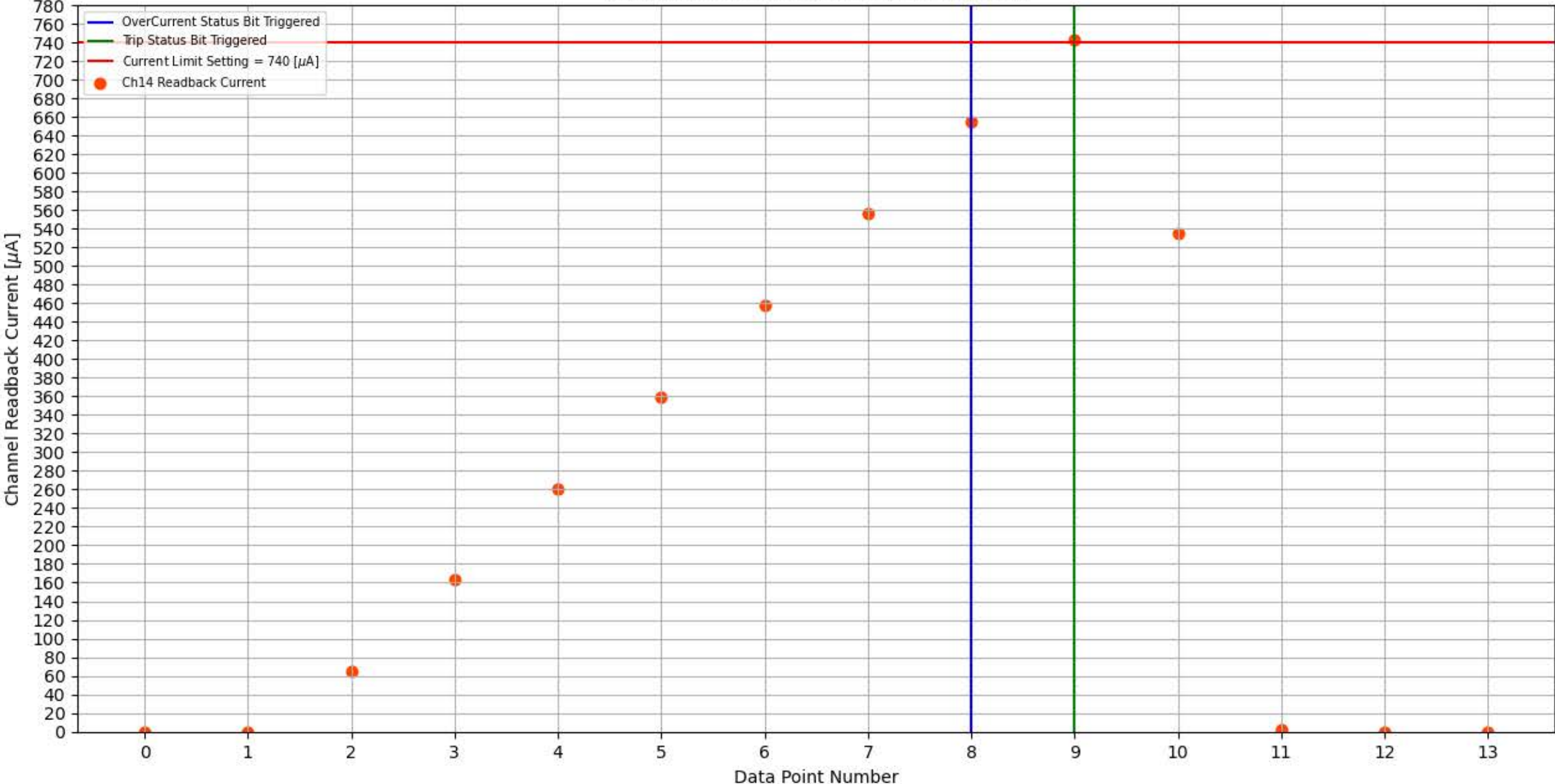
Module 313, Slot 8, Channel 14 Trip Test
