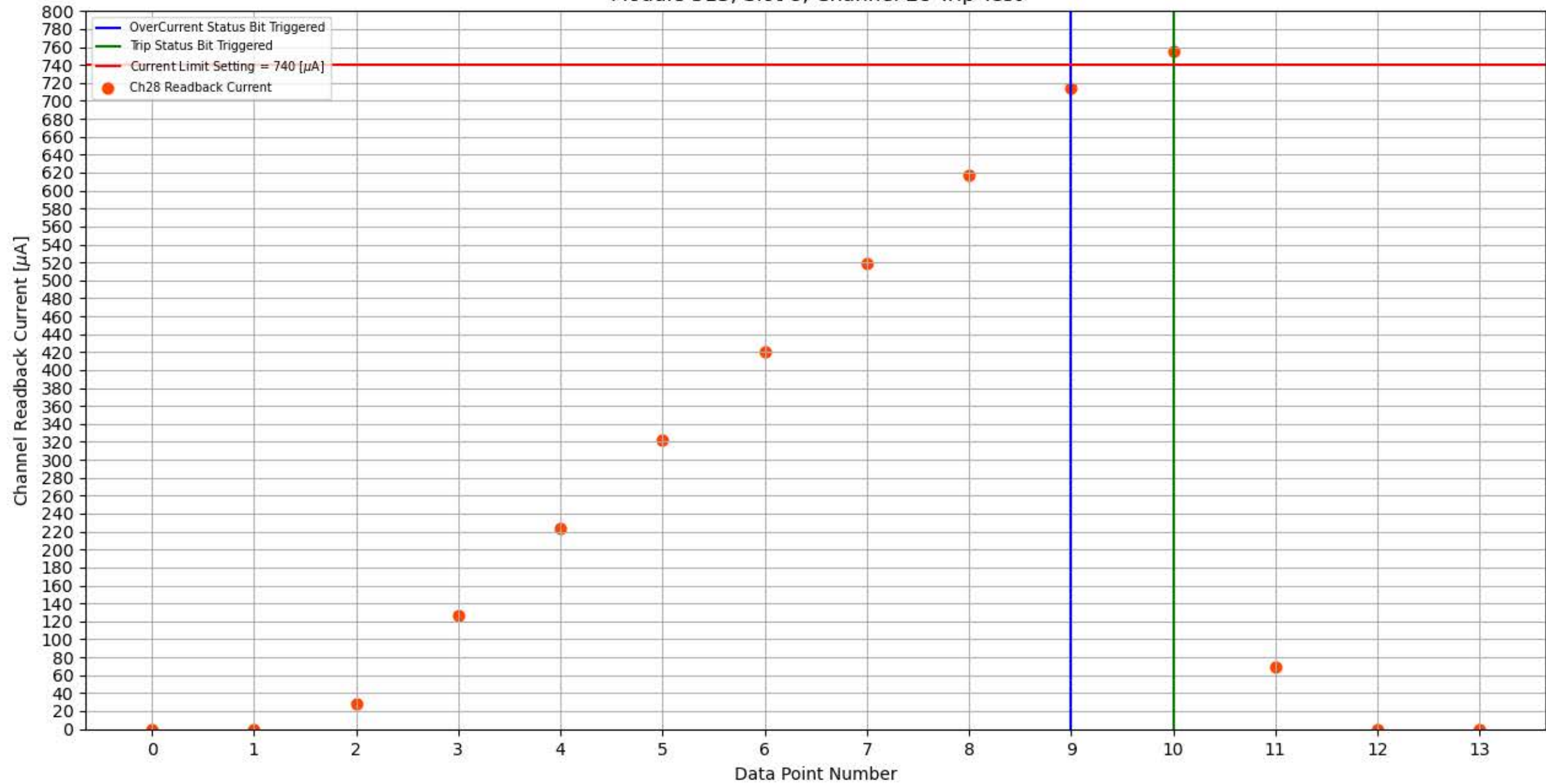
Module 313, Slot 8, Channel 28 Trip Test
