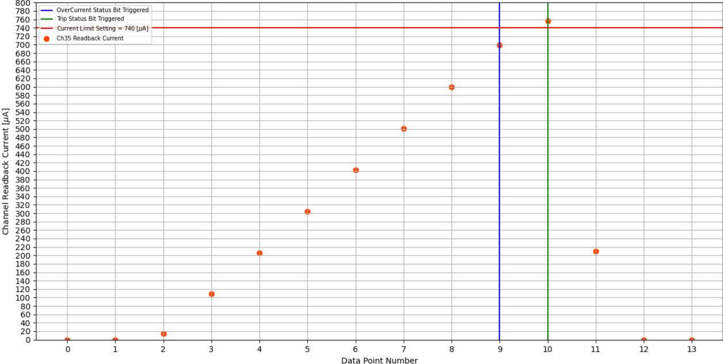
Module 313, Slot 8, Channel 35 Trip Test
