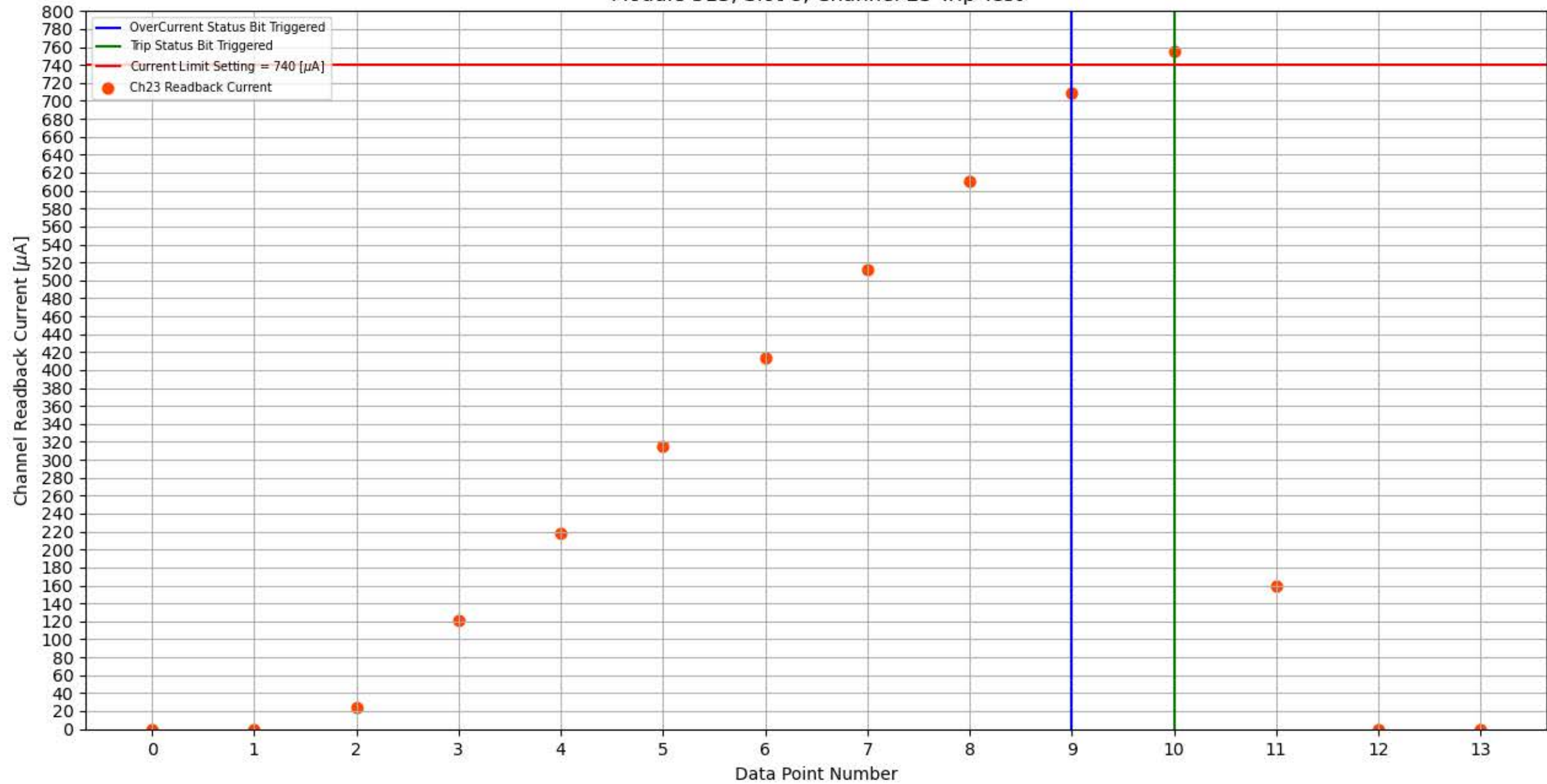
Module 313, Slot 8, Channel 23 Trip Test
