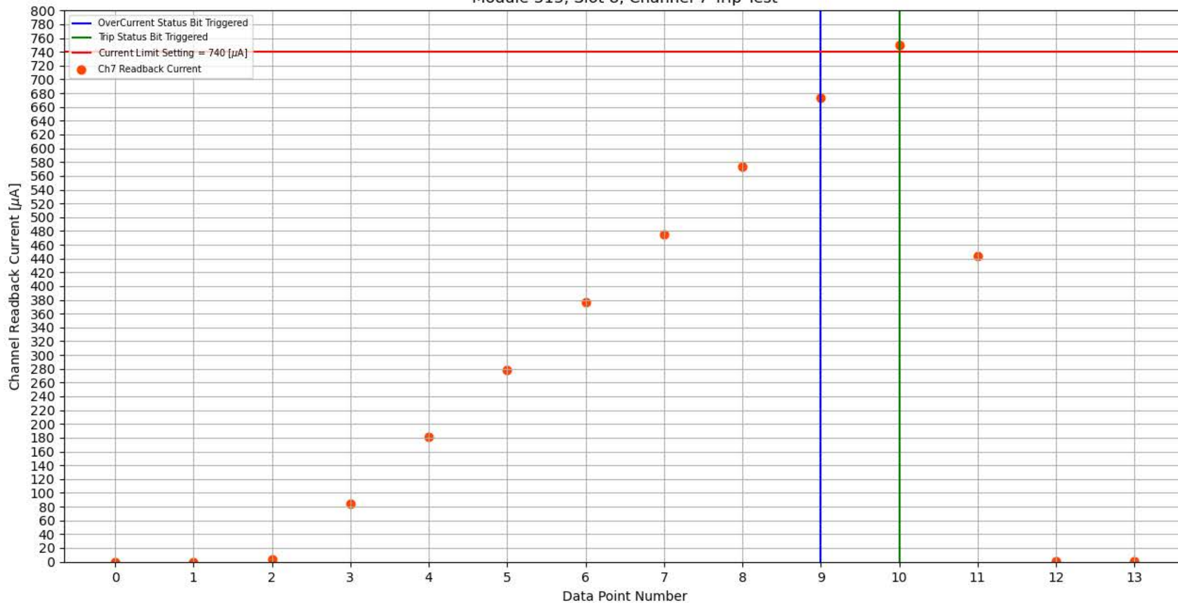
Module 313, Slot 8, Channel 7 Trip Test
