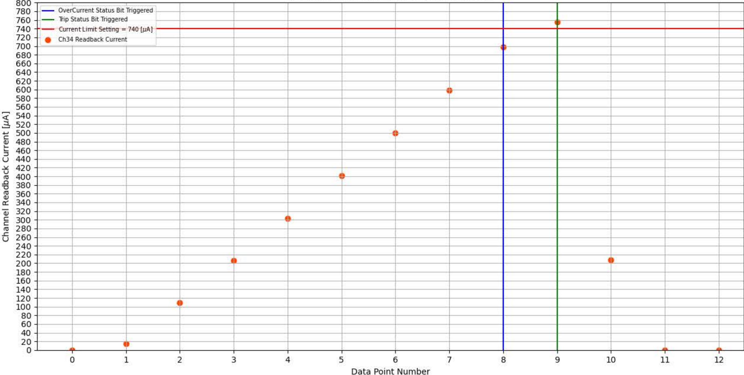
Module 313, Slot 8, Channel 34 Trip Test
