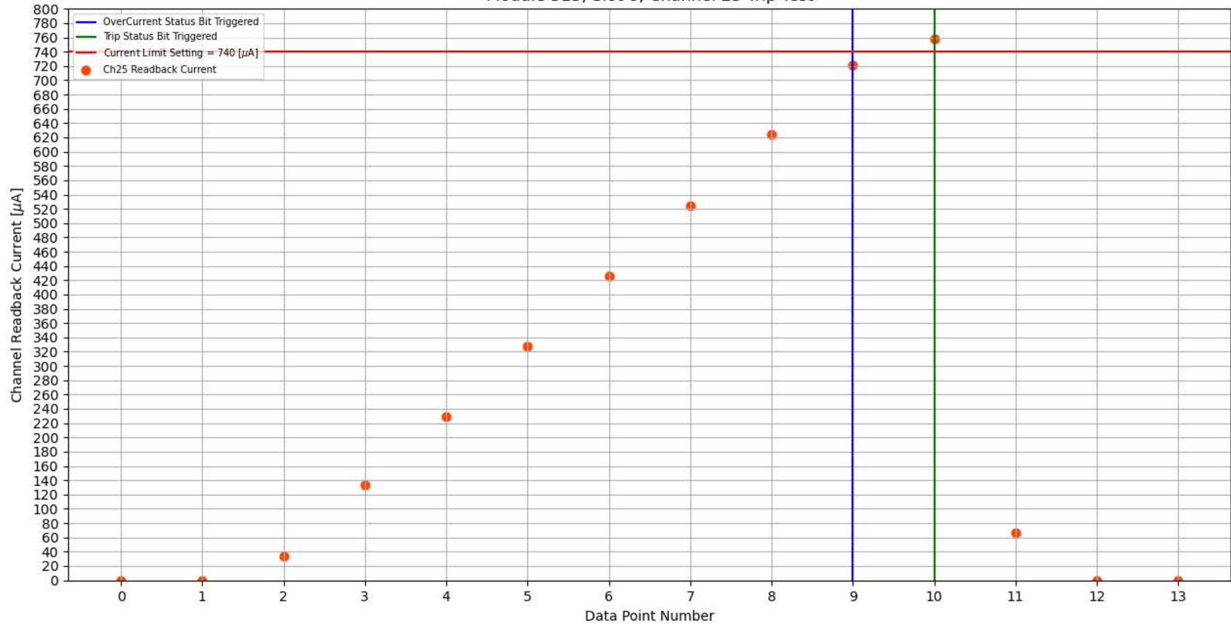
Module 313, Slot 8, Channel 25 Trip Test
