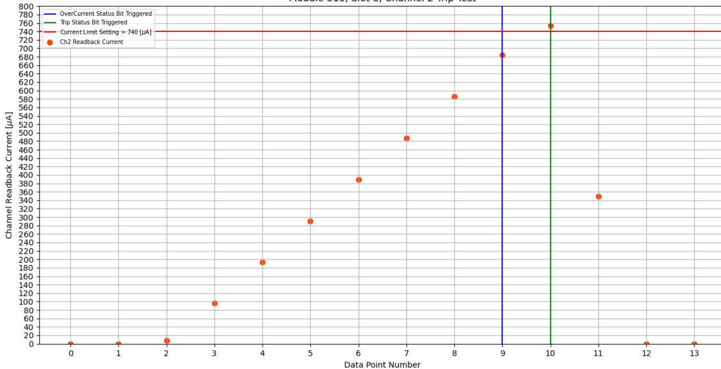
Module 313, Slot 8, Channel 2 Trip Test
