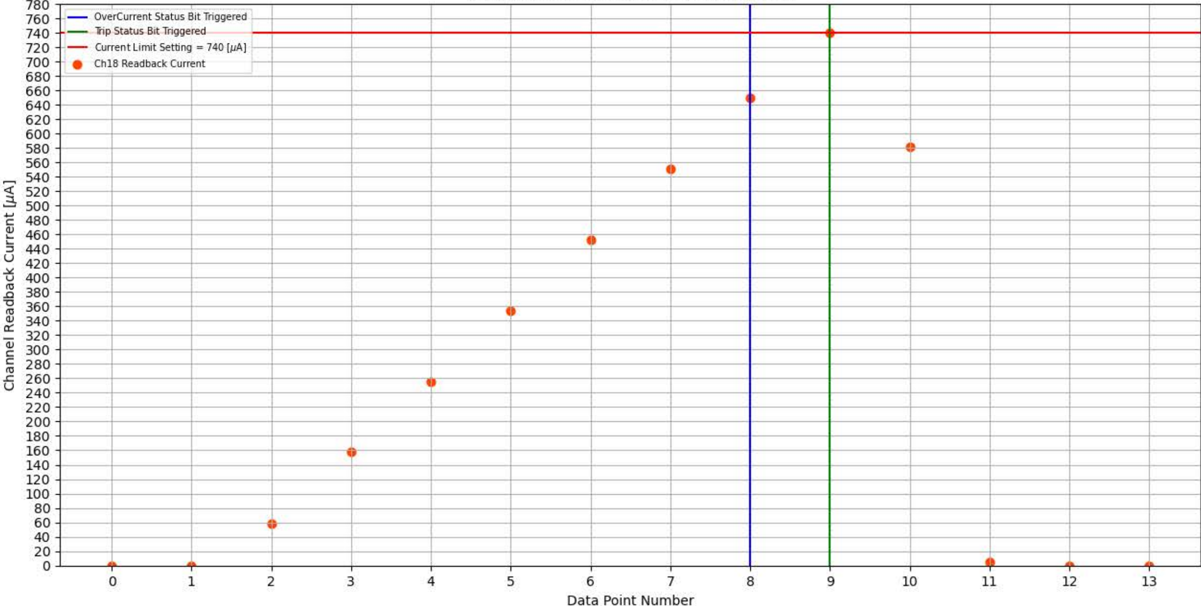
Module 313, Slot 8, Channel 18 Trip Test
