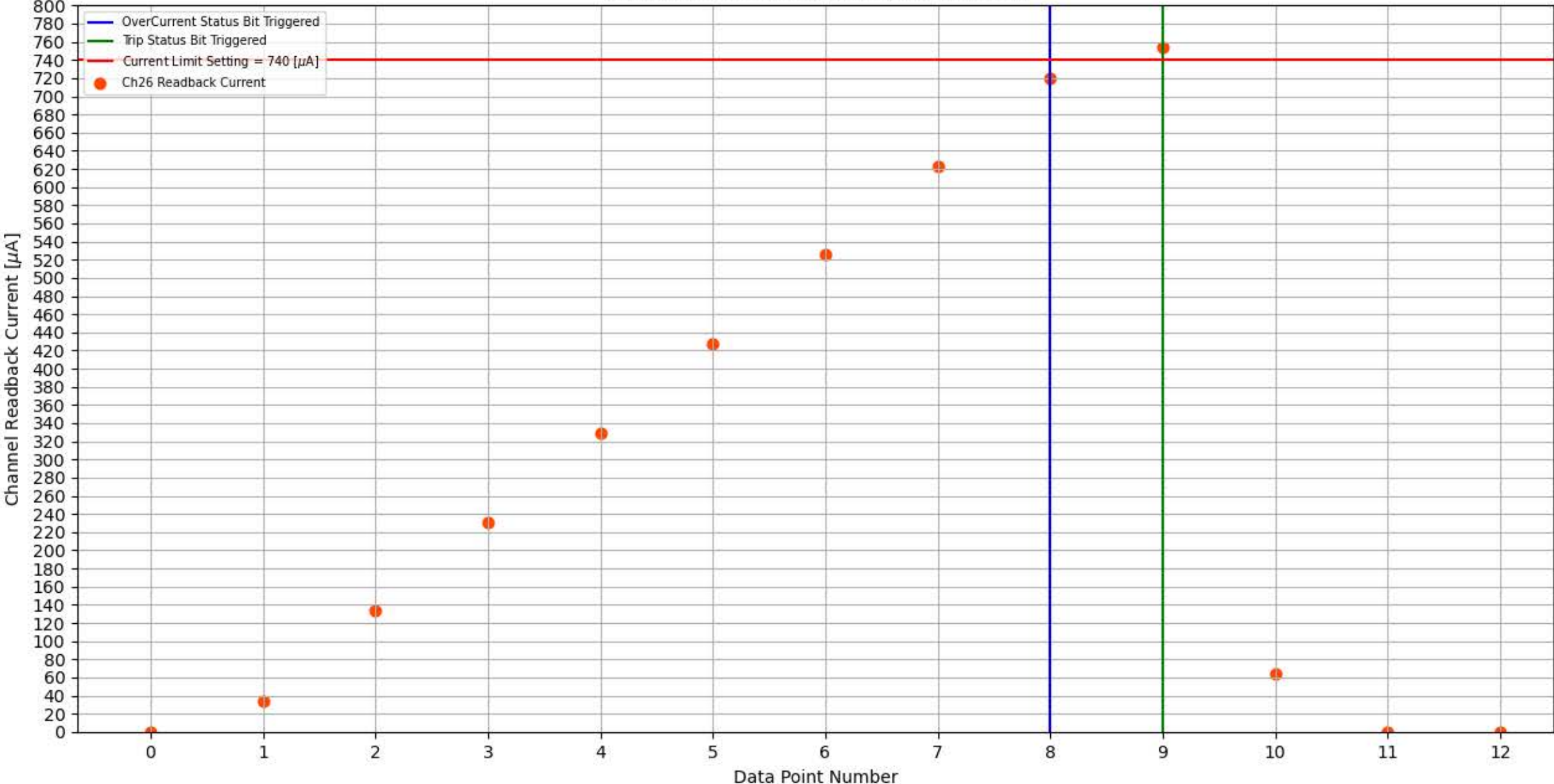
Module 313, Slot 8, Channel 26 Trip Test
