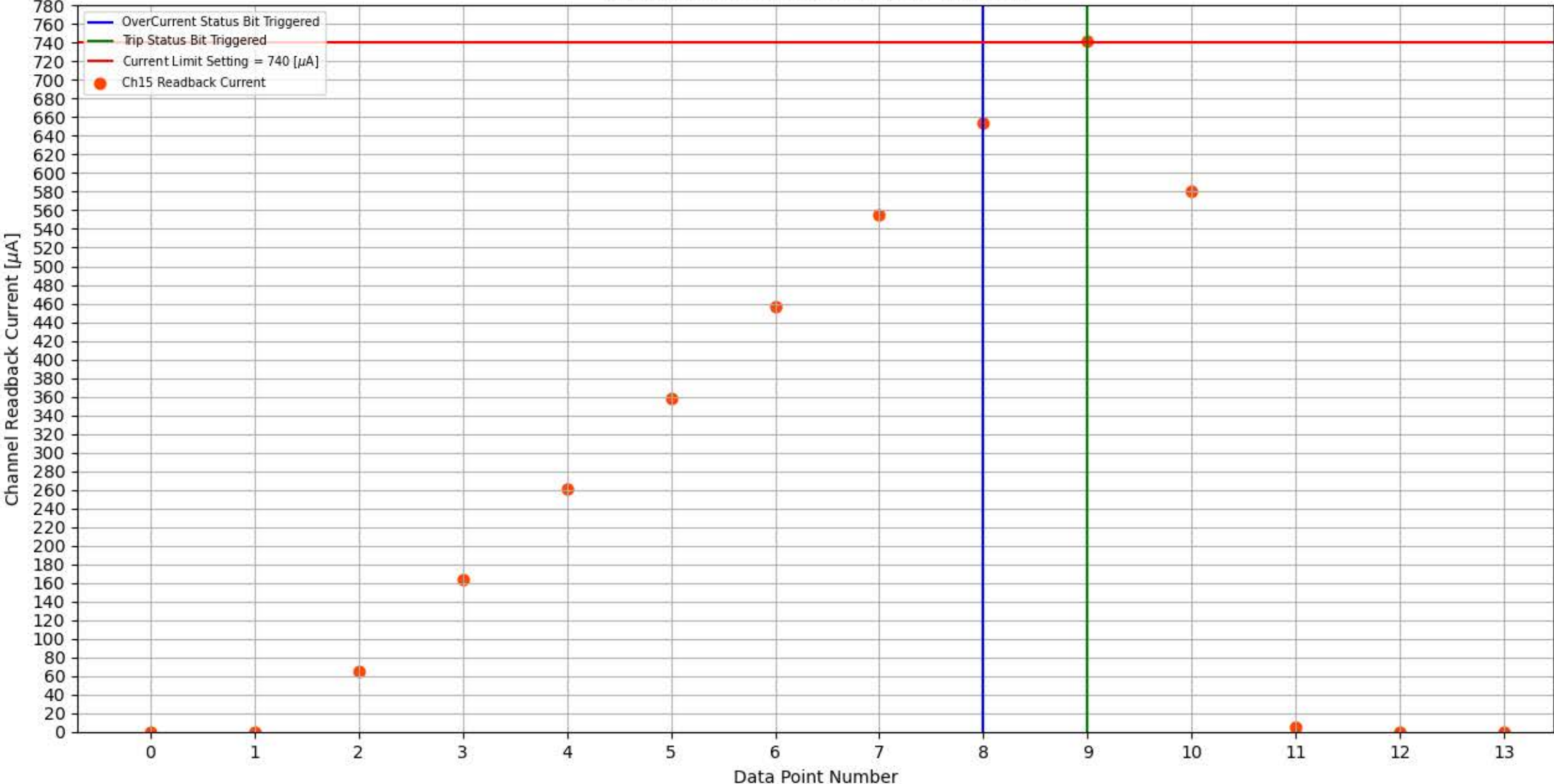
Module 313, Slot 8, Channel 15 Trip Test
