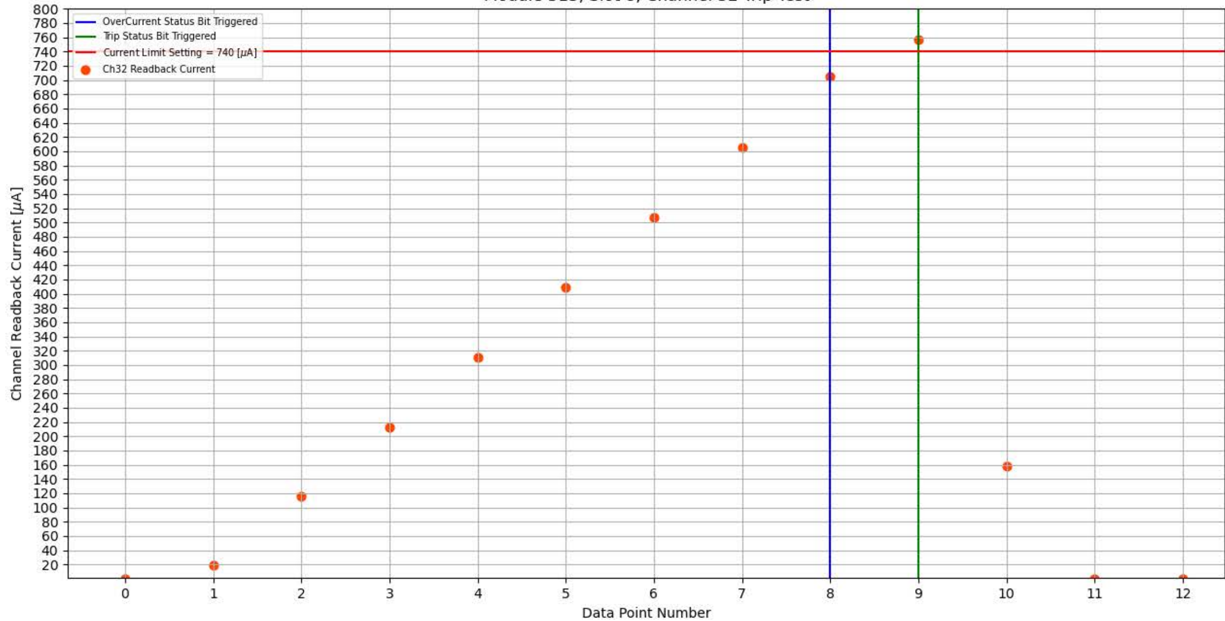
Module 313, Slot 8, Channel 32 Trip Test
