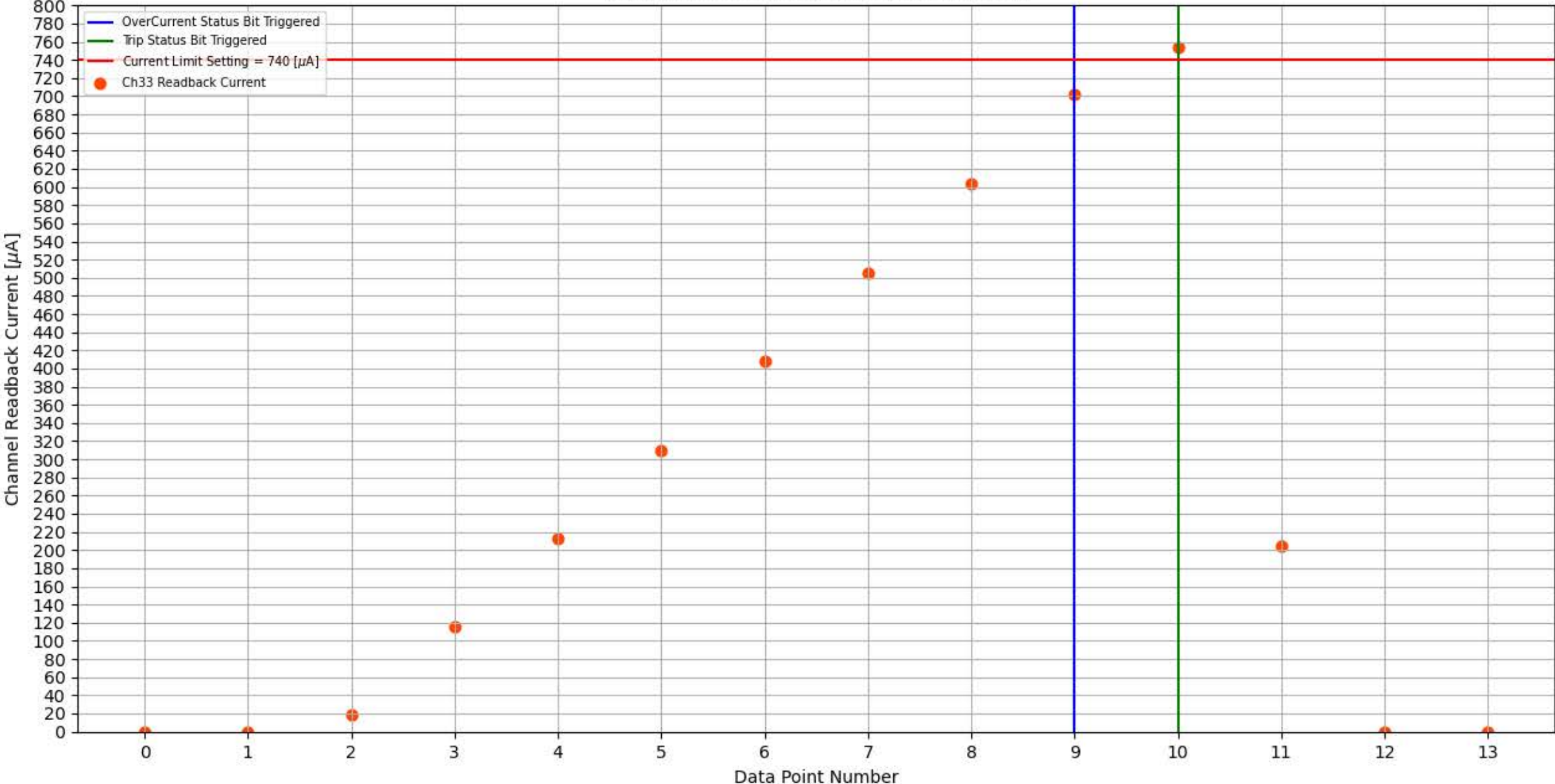
Module 313, Slot 8, Channel 33 Trip Test
