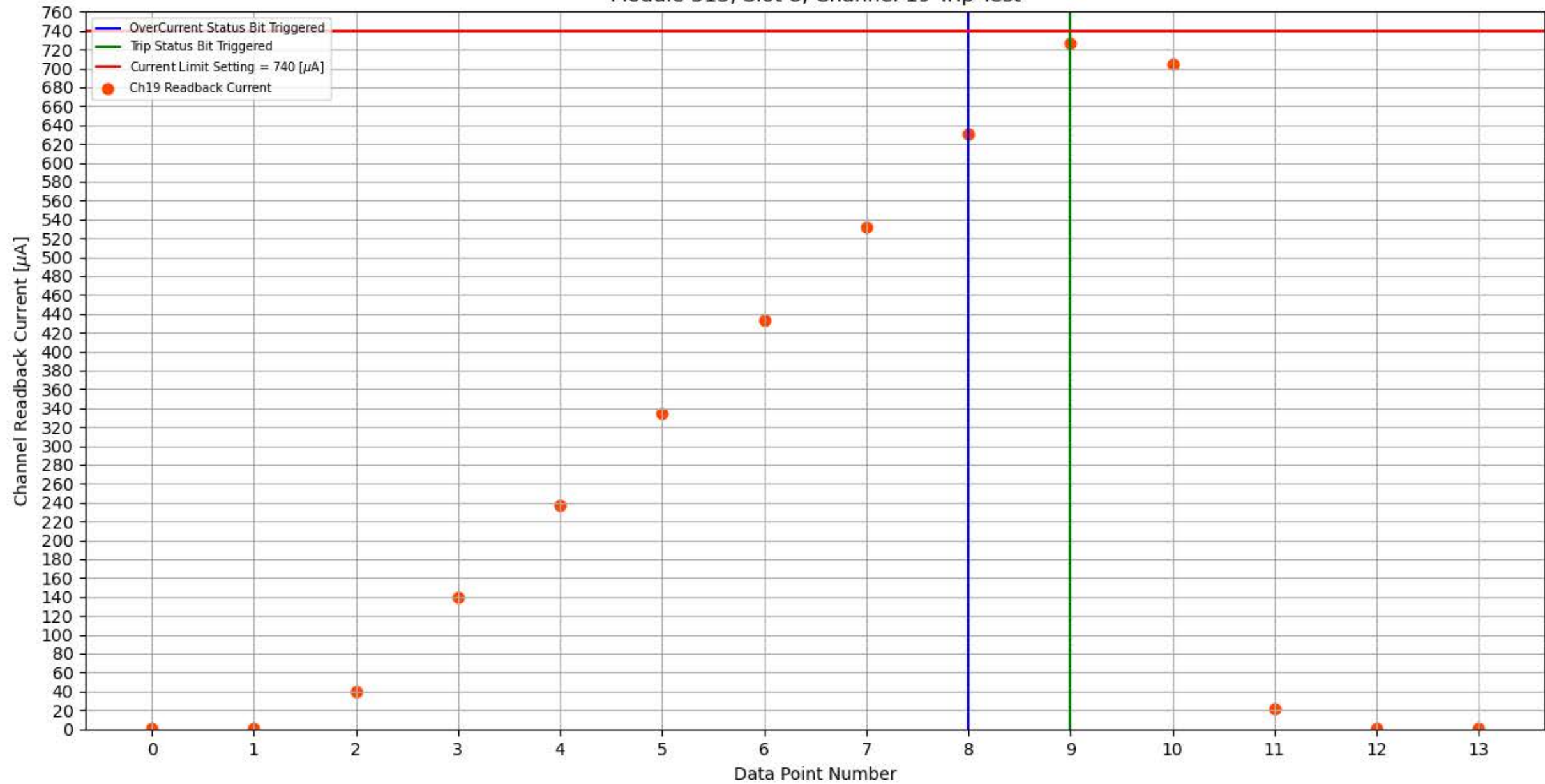
Module 313, Slot 8, Channel 19 Trip Test
