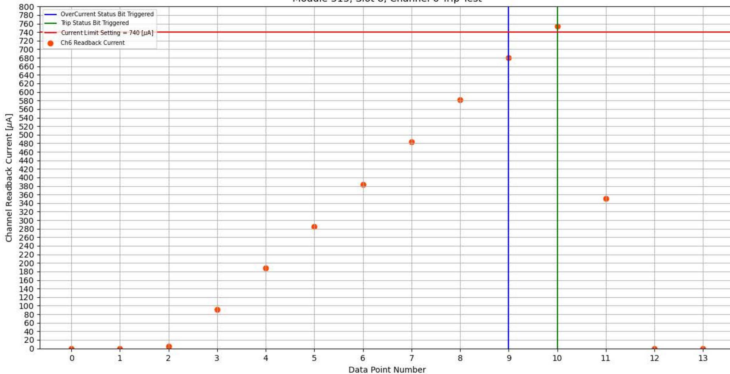
Module 313, Slot 8, Channel 6 Trip Test
