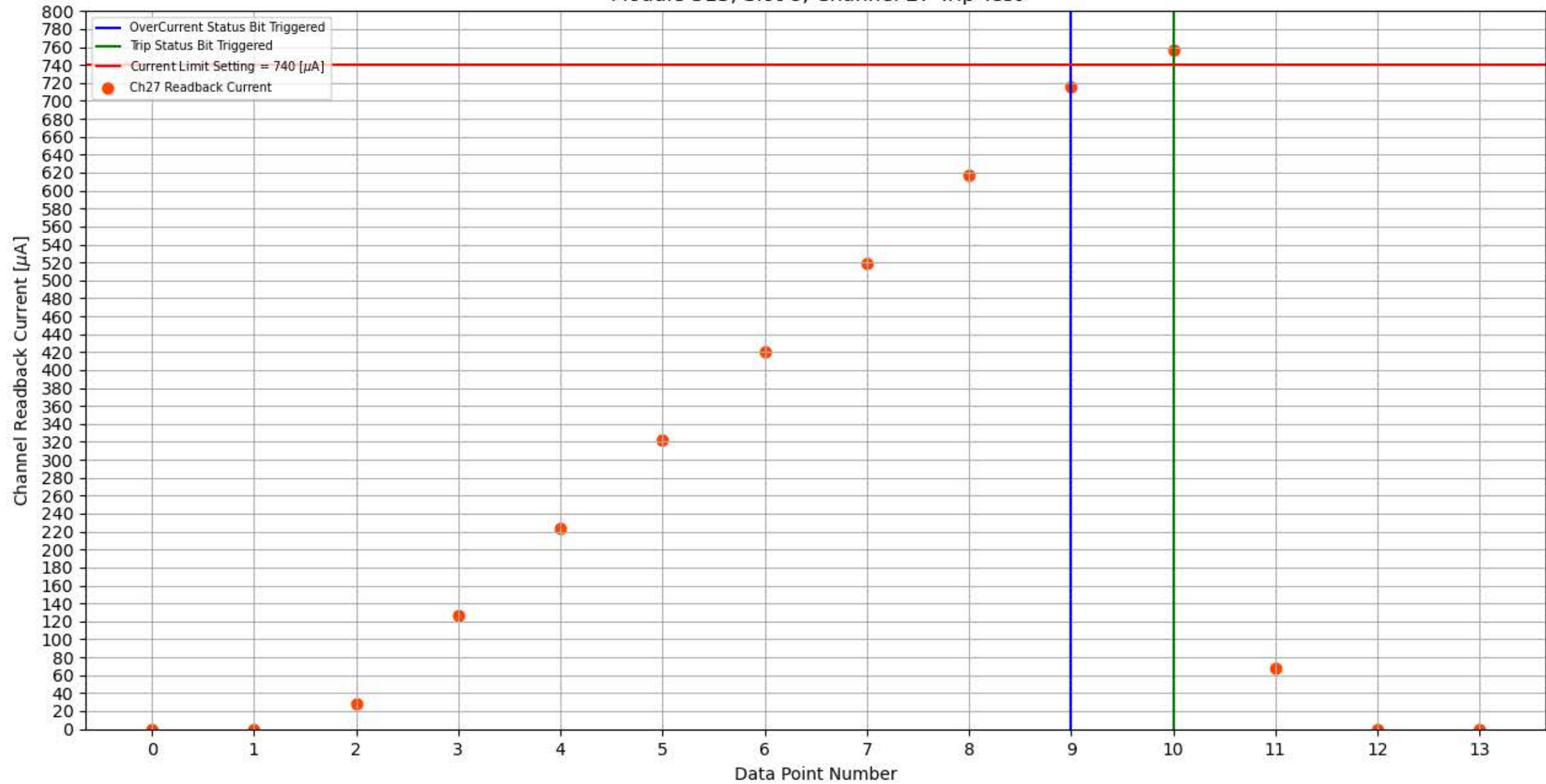
Module 313, Slot 8, Channel 27 Trip Test
