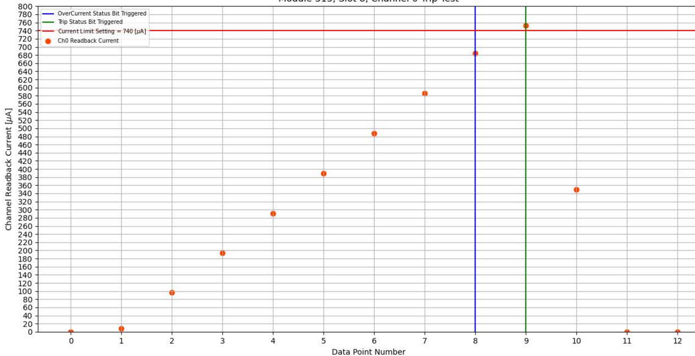
Module 313, Slot 8, Channel 0 Trip Test
