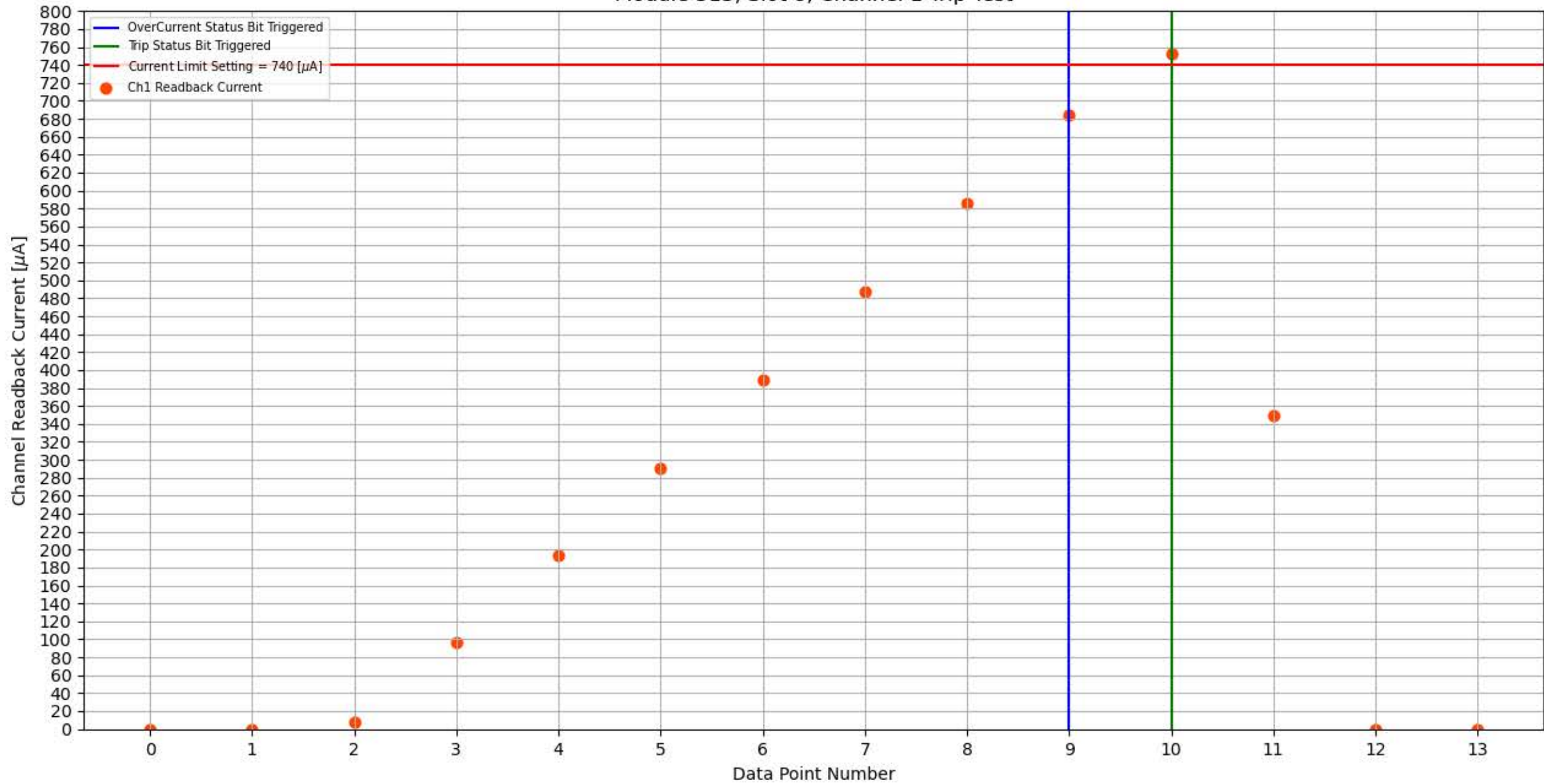
Module 313, Slot 8, Channel 1 Trip Test
