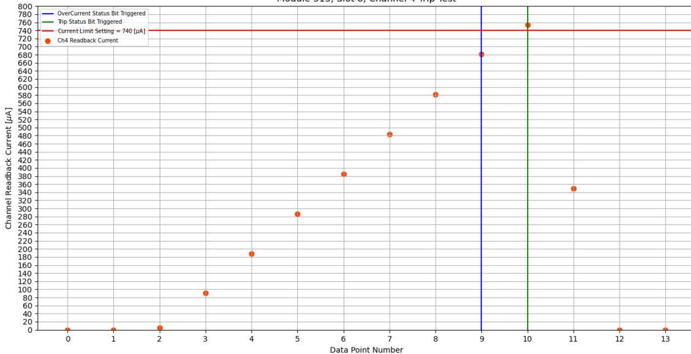
Module 313, Slot 8, Channel 4 Trip Test
