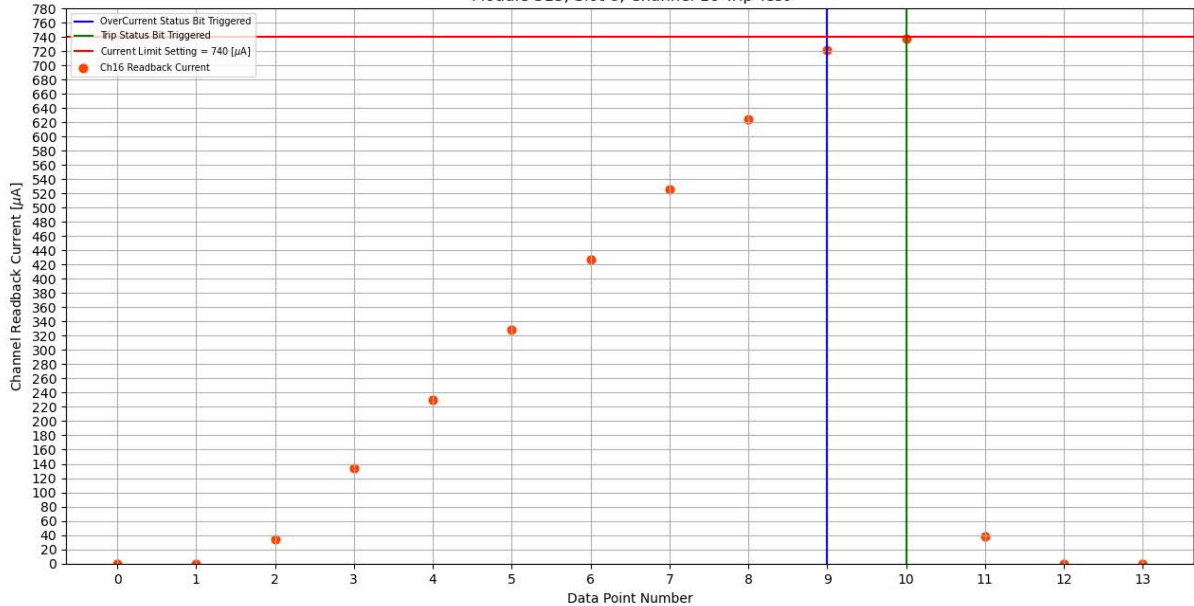
Module 313, Slot 8, Channel 16 Trip Test
