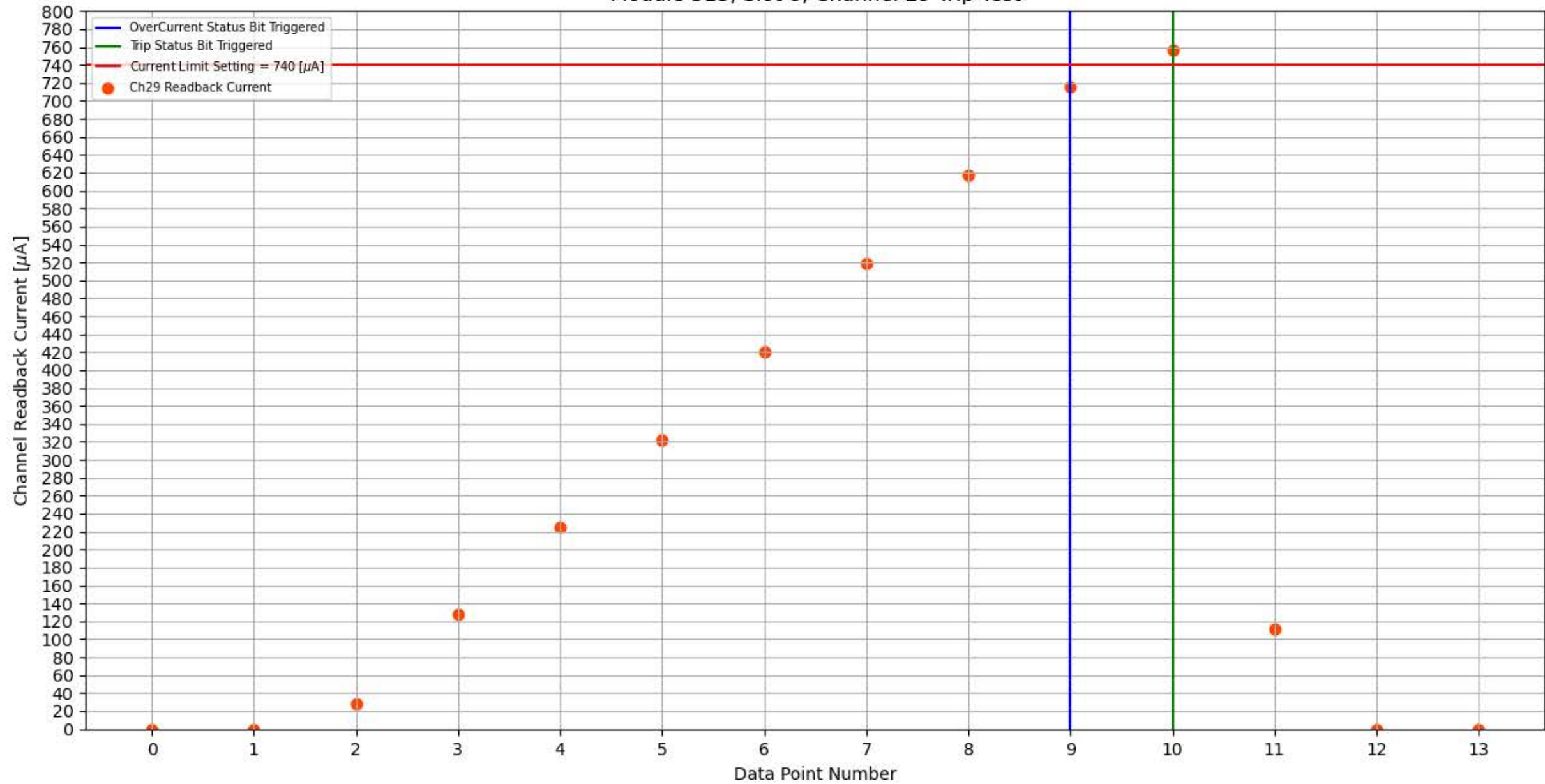
Module 313, Slot 8, Channel 29 Trip Test
