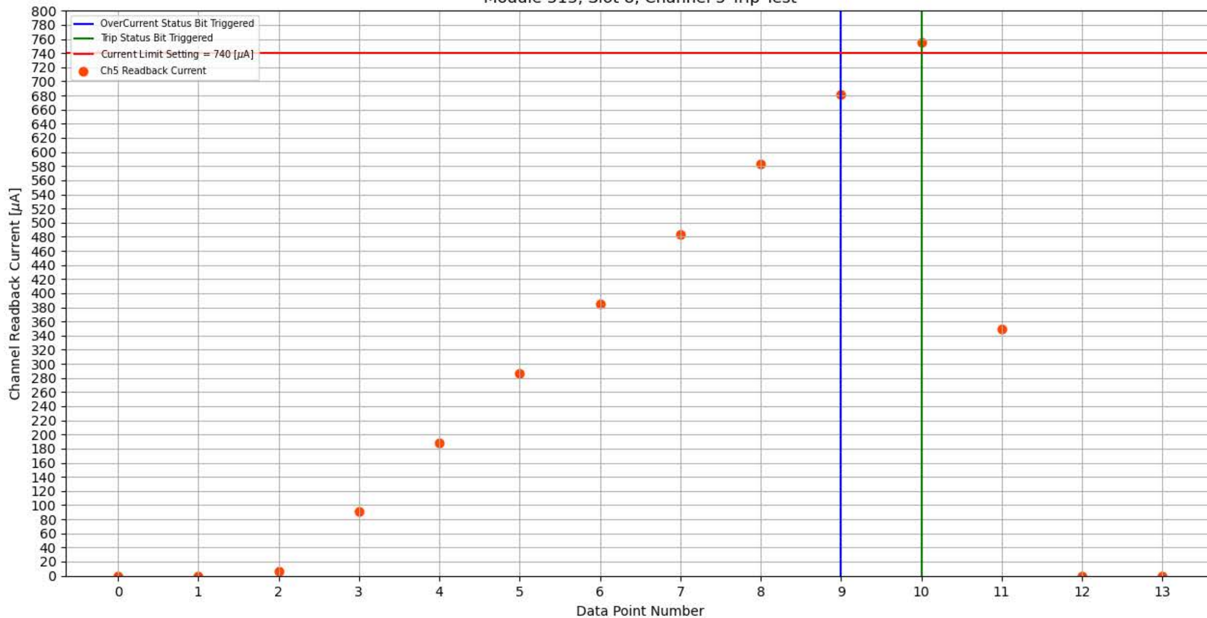
Module 313, Slot 8, Channel 5 Trip Test
