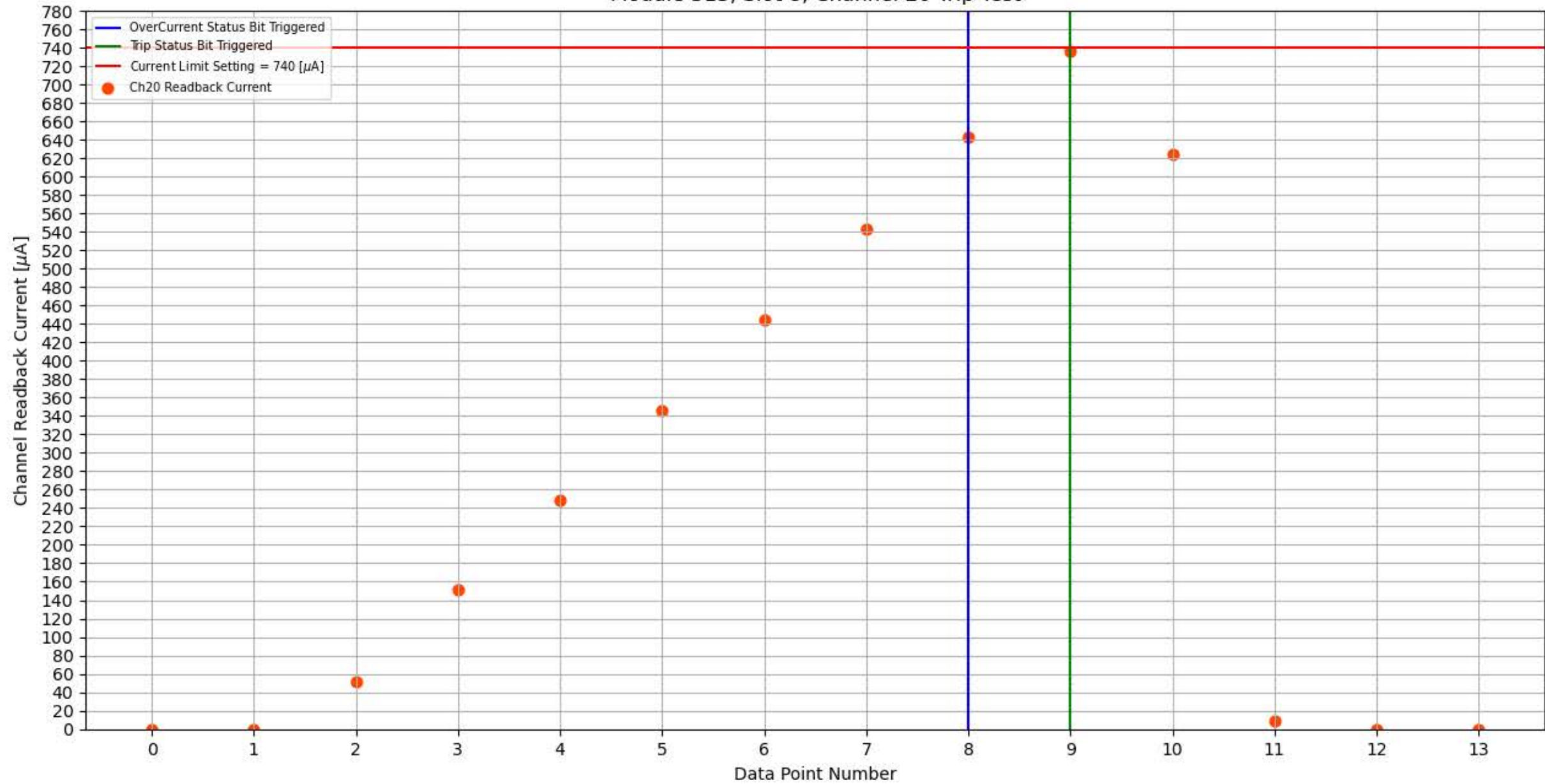
Module 313, Slot 8, Channel 20 Trip Test
